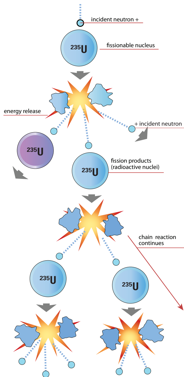
FIG. 7: Nuclear fission
